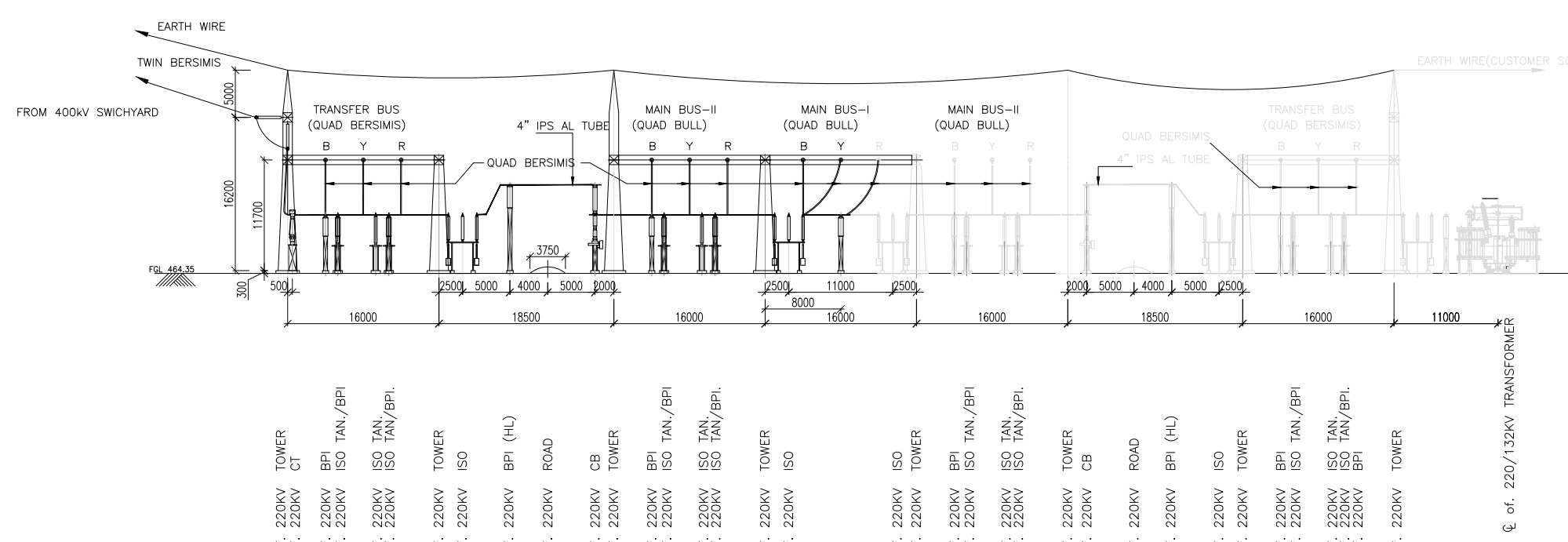
SECTION-2F-2F (400/220KV ICT-TIE-220/132KV ICT (F))
