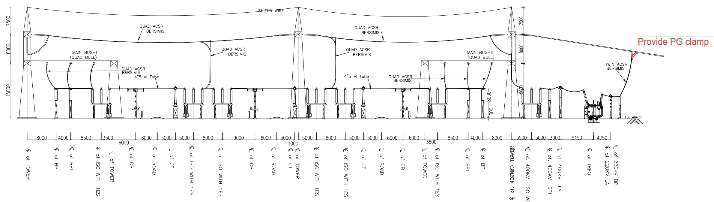
SECTION 4C-4C (765/400KV ICT 2-TIE-400/220KV ICT-1) SECTION 4D-4D (765/400KV ICT 1-TIE-400/220KV ICT-2)
