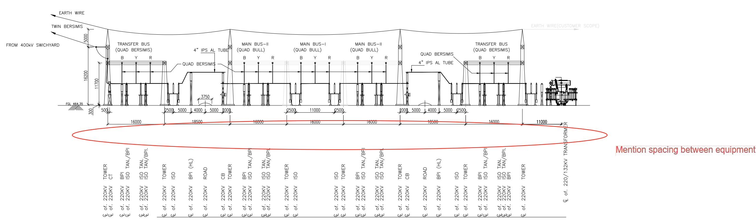
SECTION-2E-2E (400/220KV ICT-TIE-220/132KV ICT)
