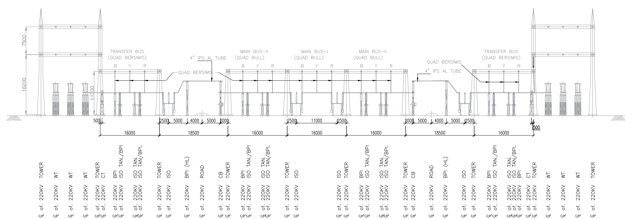
SECTION 2A-2A (220KV LINE.1-TIE-LINE.2)
