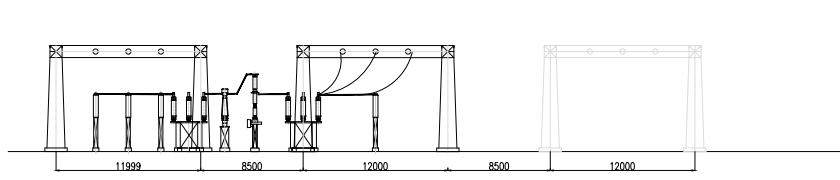
132KV Section 1A-1A(TBC)
