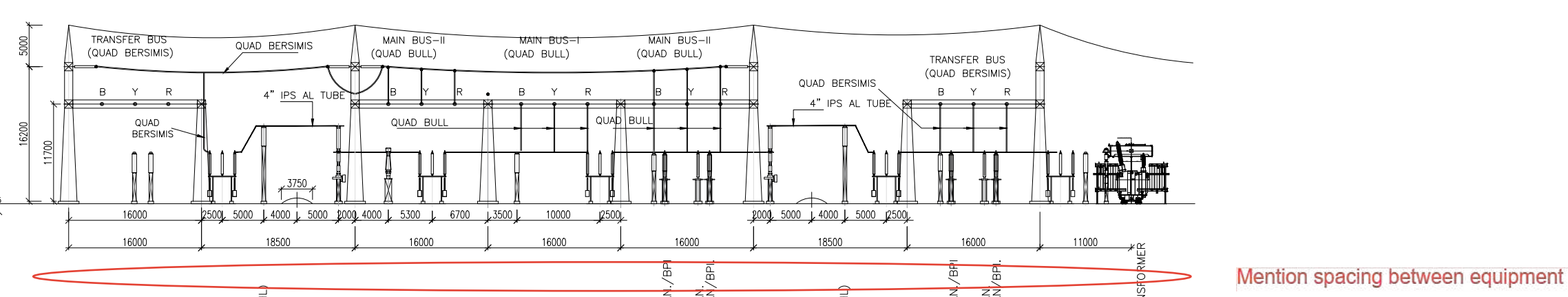
SECTION-2C-2C (220KV-BUS COUPLER-TIE-1)
