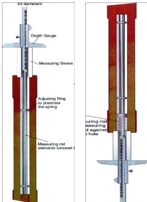
Expansion measuring device / scale
