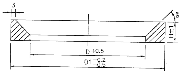
Fig: Indicative Sketch of Reinforced Gaskets
