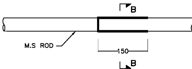
DETAIL OF CROSS JOINT
