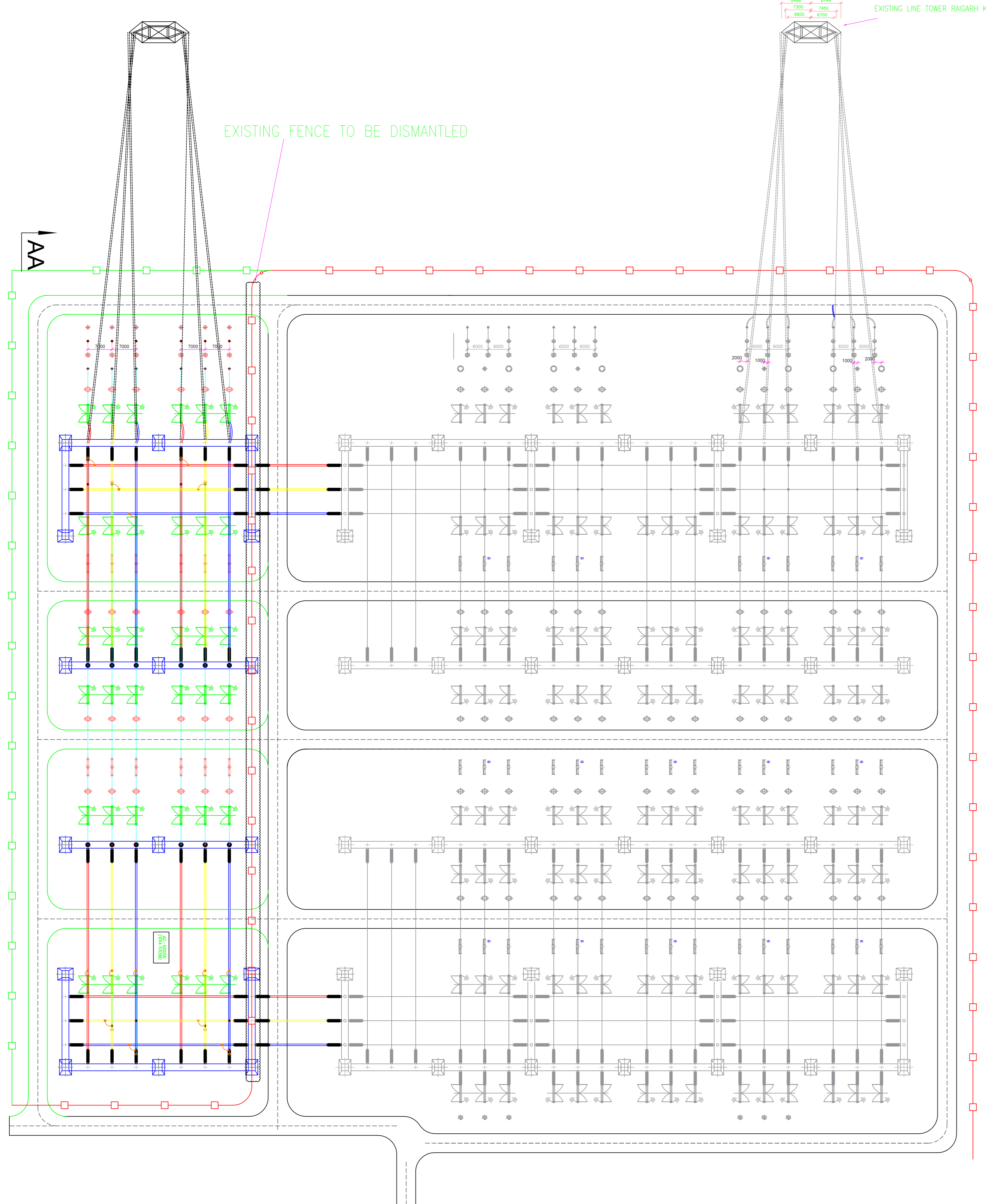
STAGE-I EXTENSION ELECTRICAL LAYOUT PLAN
