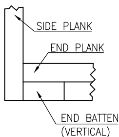
DETAIL-B (TOP-VIEW)
