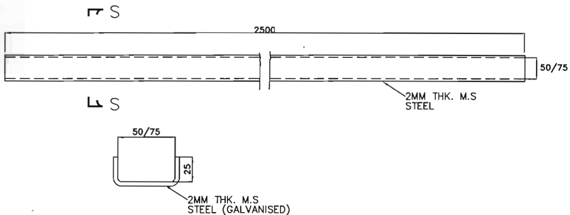
SECTION S-S
