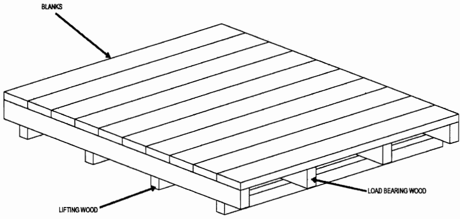
BASE FRAME
