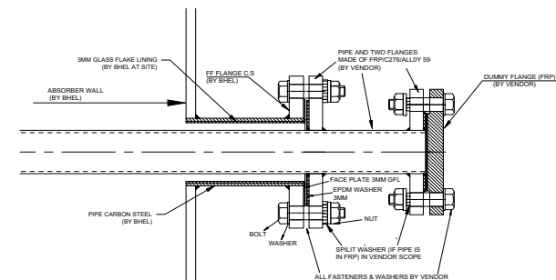
DETAIL-Z (EMERGENCY FLUSH PIPE ARRANGEMENT)
