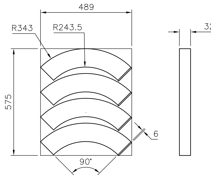
ITEM-02 CUTTING PLAN
