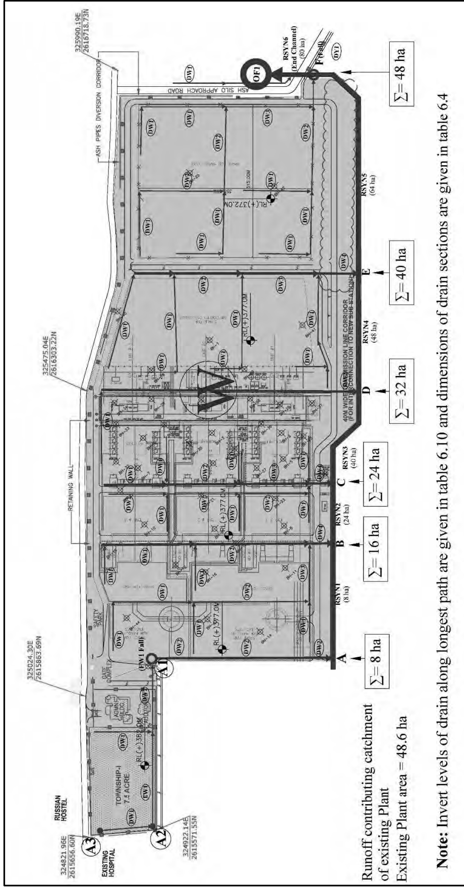
Figure 6.3 Drainage Plan Showing Plant Area Drains, Longest Flow Path and Outfall Location (FW1, F) in W Zone
