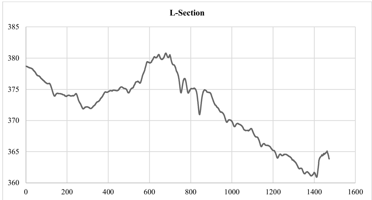
Figure 5.5: L-Section of SY nala
