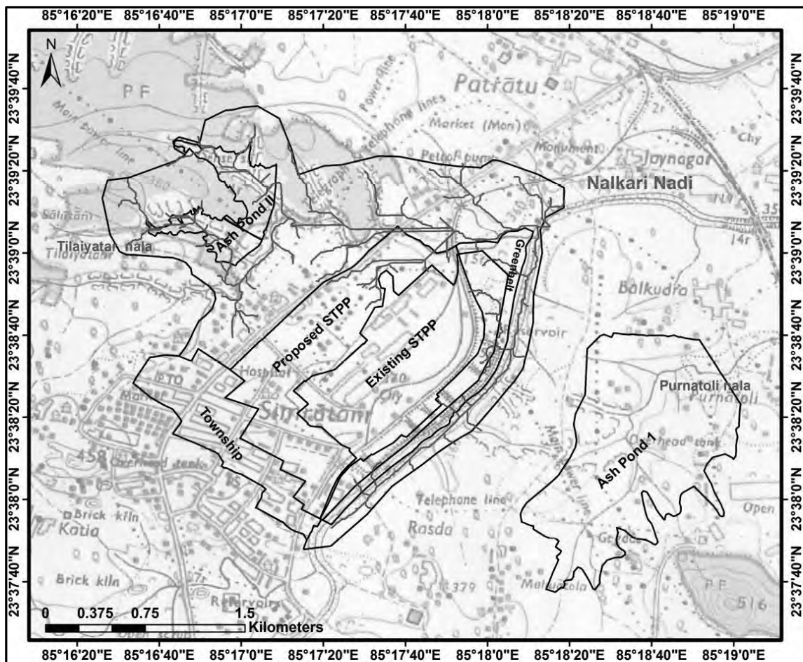
Figure 6.6: Location of ash dyke areas with reference to proposed STPP
