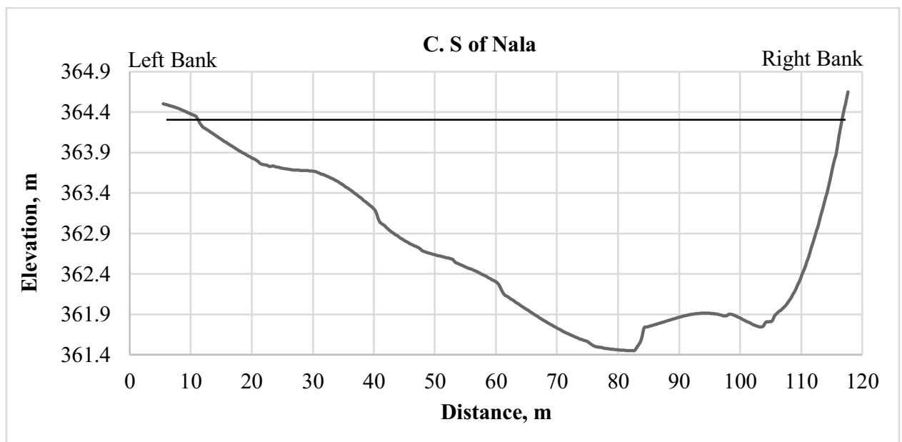
Figure 5.4: Cross section of SY nala at location
