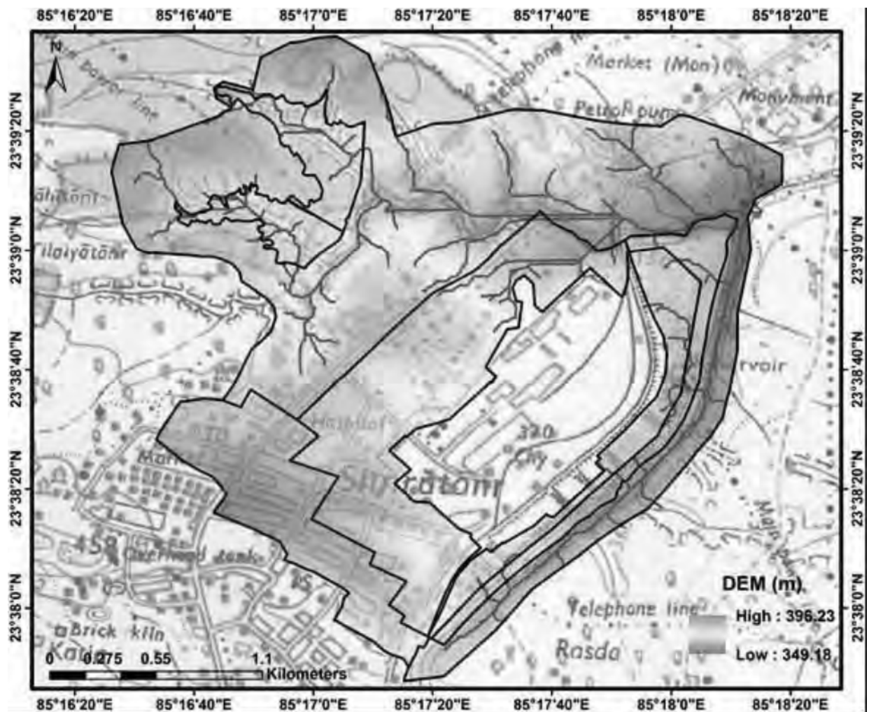
Figure 5.2: Natural drainage in vicinity of plant area HFL 367.5 m (year 1958)
