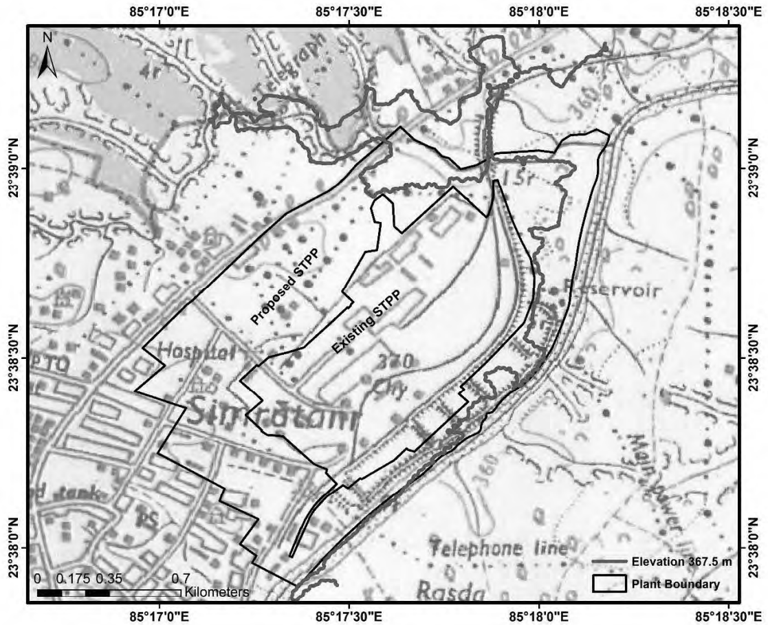
Figure 5.3: Topography of plant area and HFL 367.5 m (Flood in year 1958)
