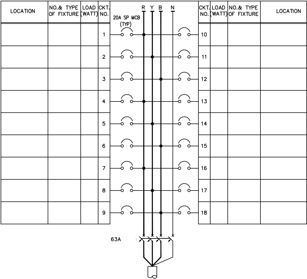
3-LINE DIAGRAM : LIGHTING PANEL
