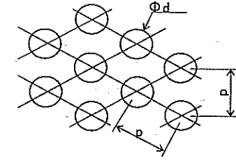
PUNCHING METAL DETAIL
