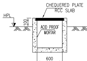
TYP. TRENCH SECTION
