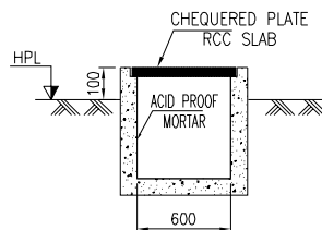
TYP. TRENCH SECTION
