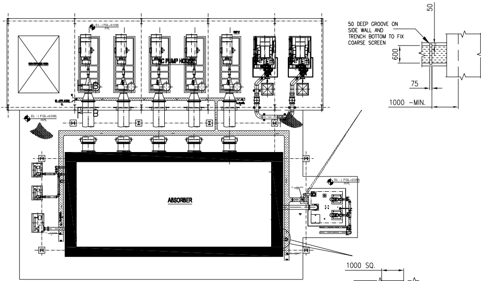
TYPICAL DRAIN TRENCH LAYOUT NEAR ABSORBER
