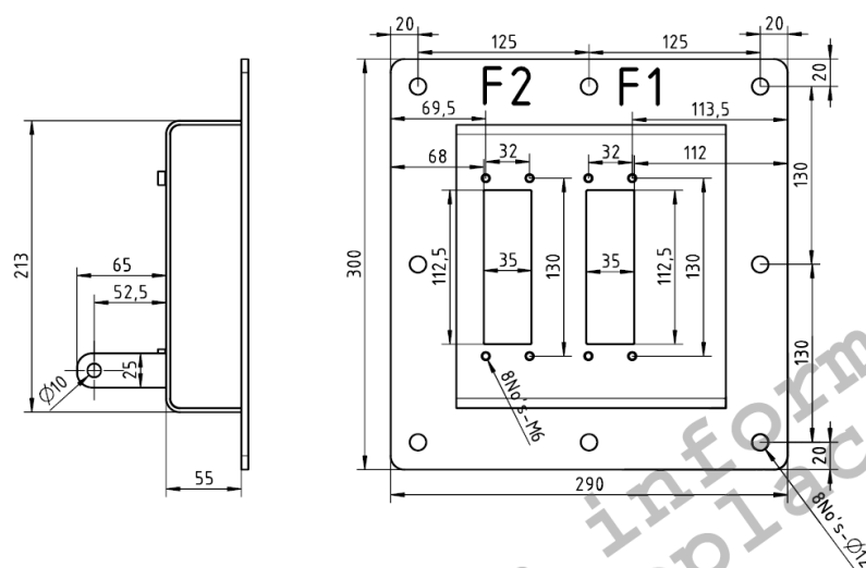
(ix) F1,F2 Coupler Plate – Mirror Orientation
