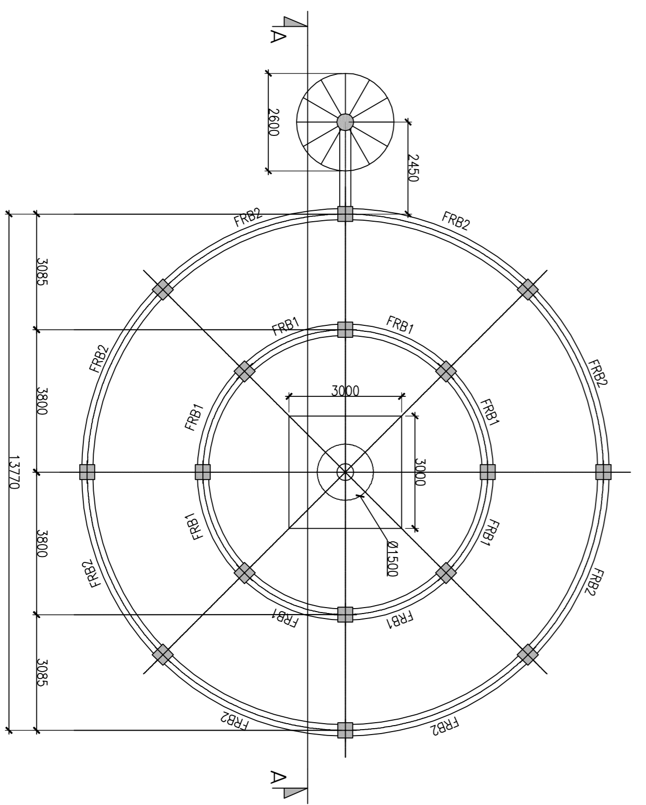
PLAN AT EL. +15.00 SCALE 1:100
