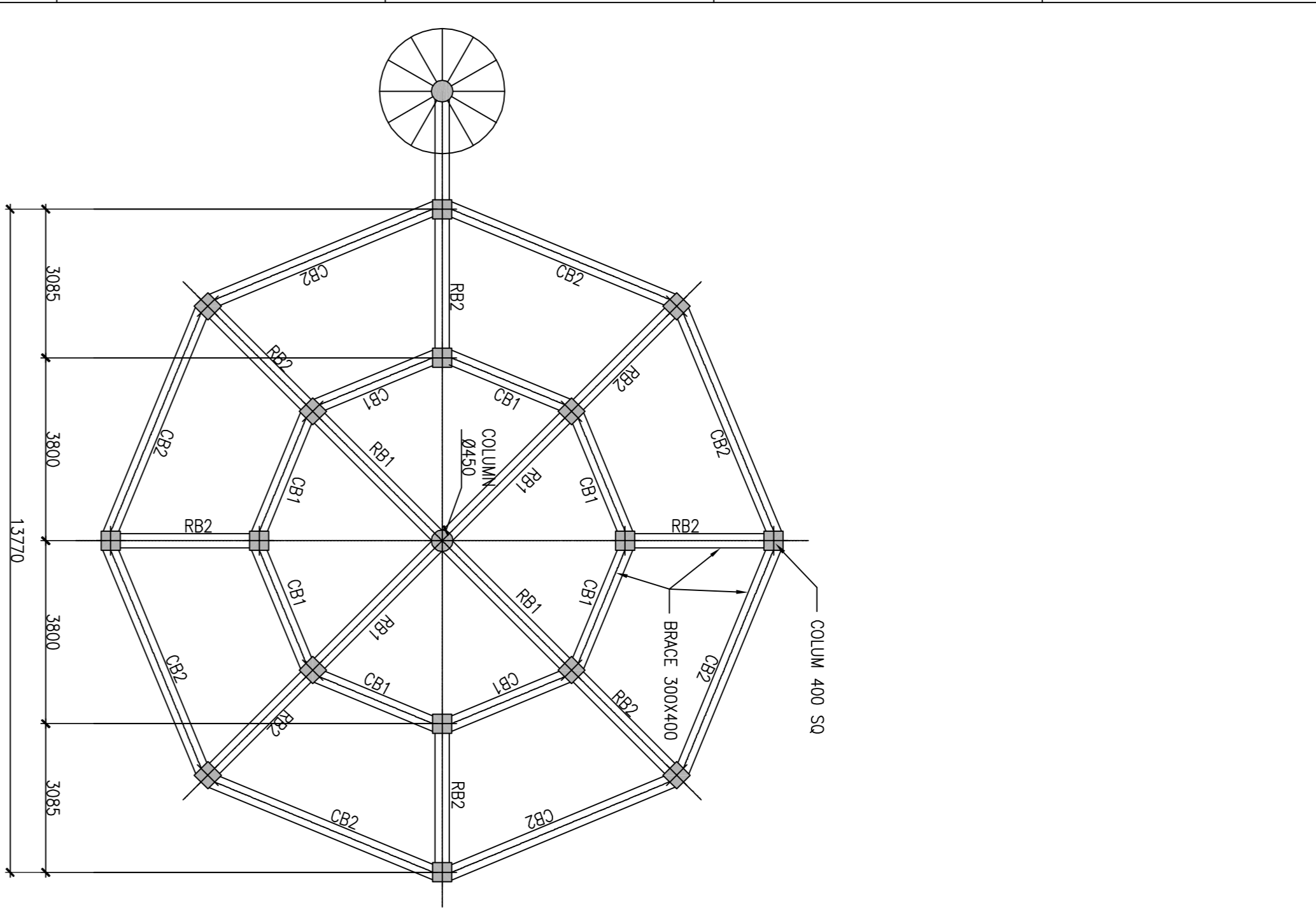
PLAN AT EL. +3.00 & +9.00 SCALE 1:100
