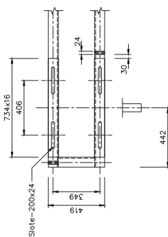
(MOTOR SLIDE RAIL DETAIL)
