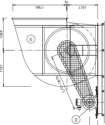
DRIVE END ELEVATION
