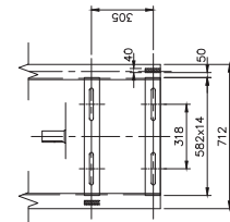
(MOTOR SLIDE RAIL DETAIL)
