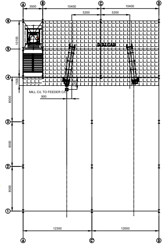
PLAN VIEW OF EL(+12.2M). FEEDER FLOOR
