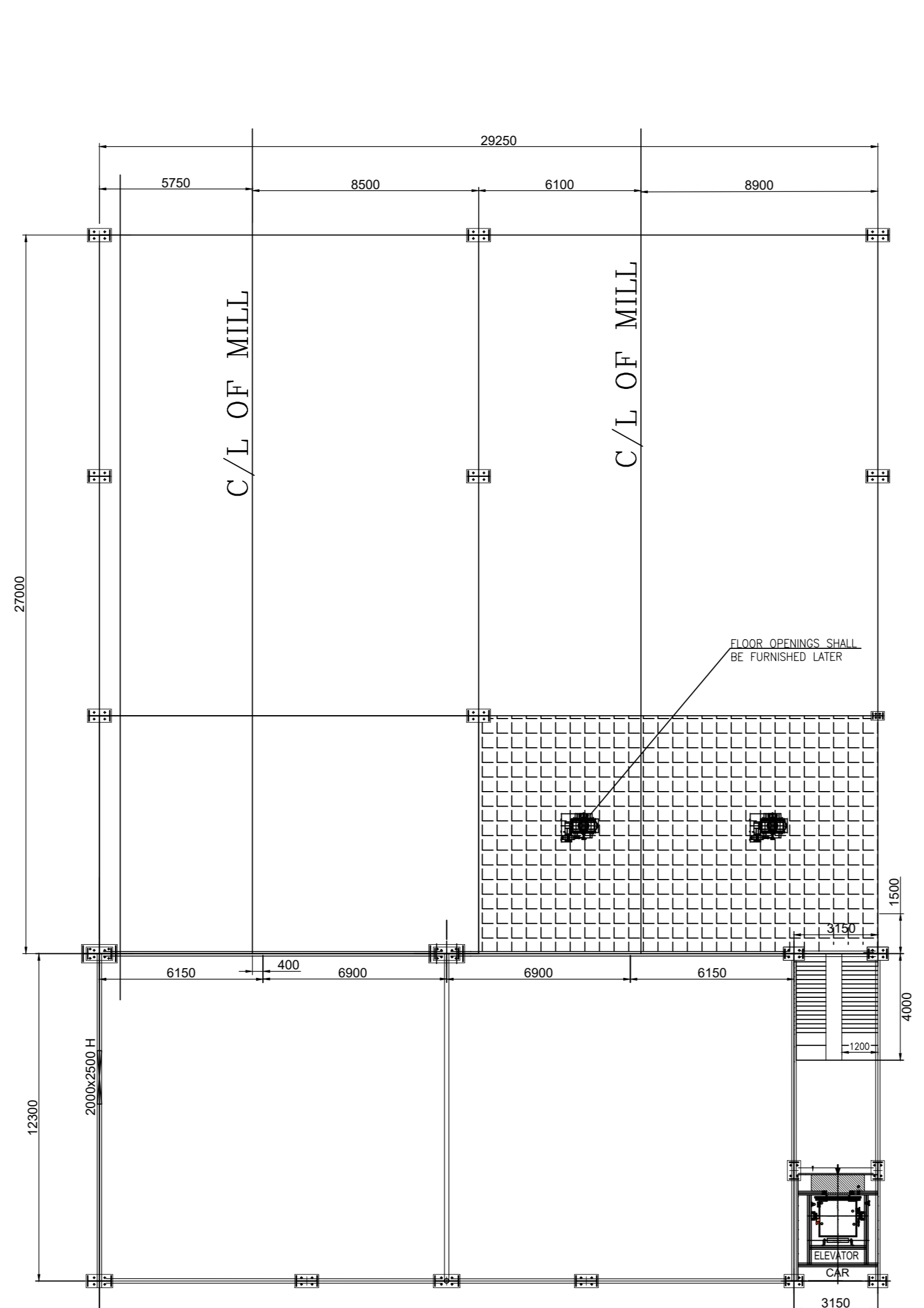
PLAN VIEW OF EL(+).24.5M ACCESS TO DISTRIBUTION BOX FLOOR
