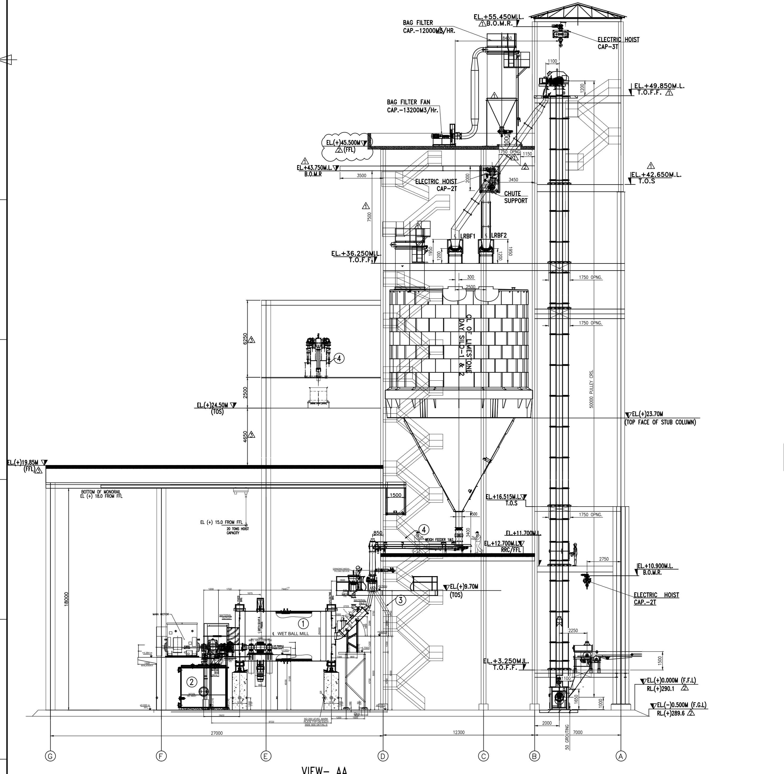
VIEW-AA
