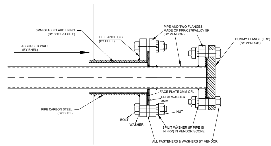
DETAIL-Z (EMERGENCY FLUSH PIPE ARRANGEMENT)
