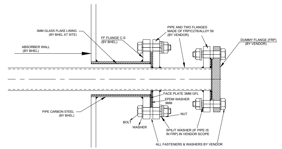
DETAIL-Z (EMERGENCY FLUSH PIPE ARRANGEMENT)
