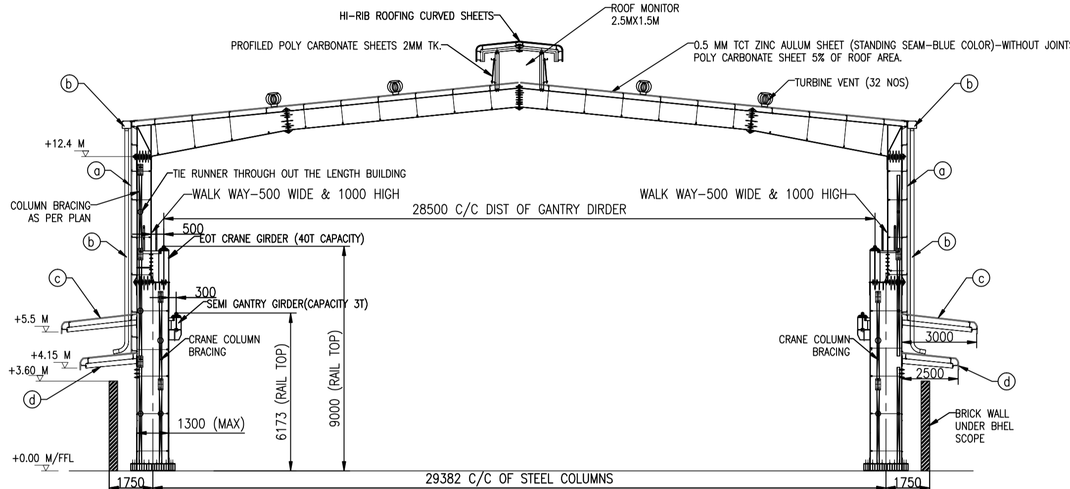
SECTION AA
