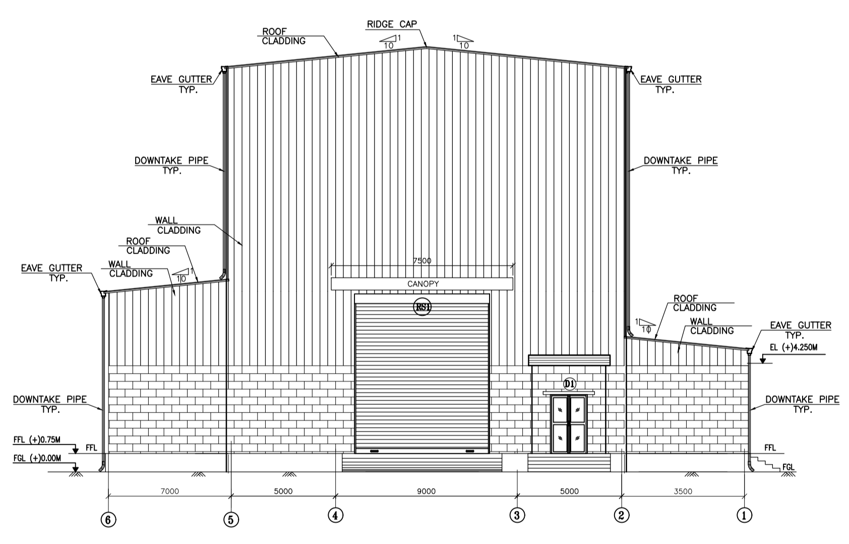
ELEVATION -C
