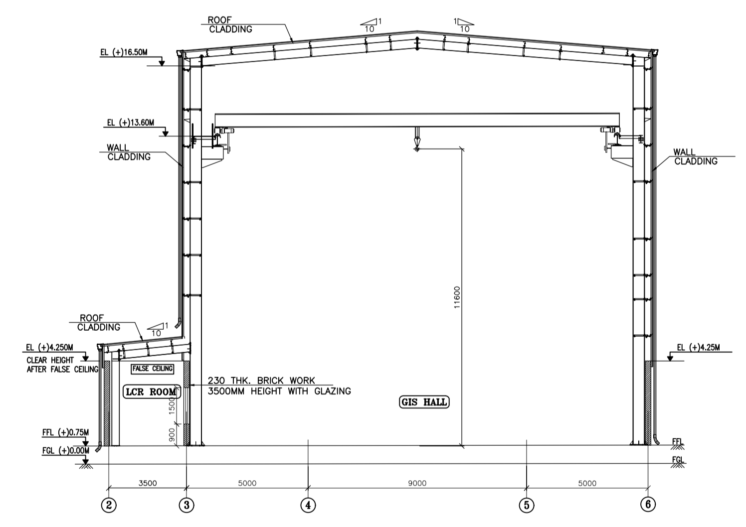
SECTION 2-2
