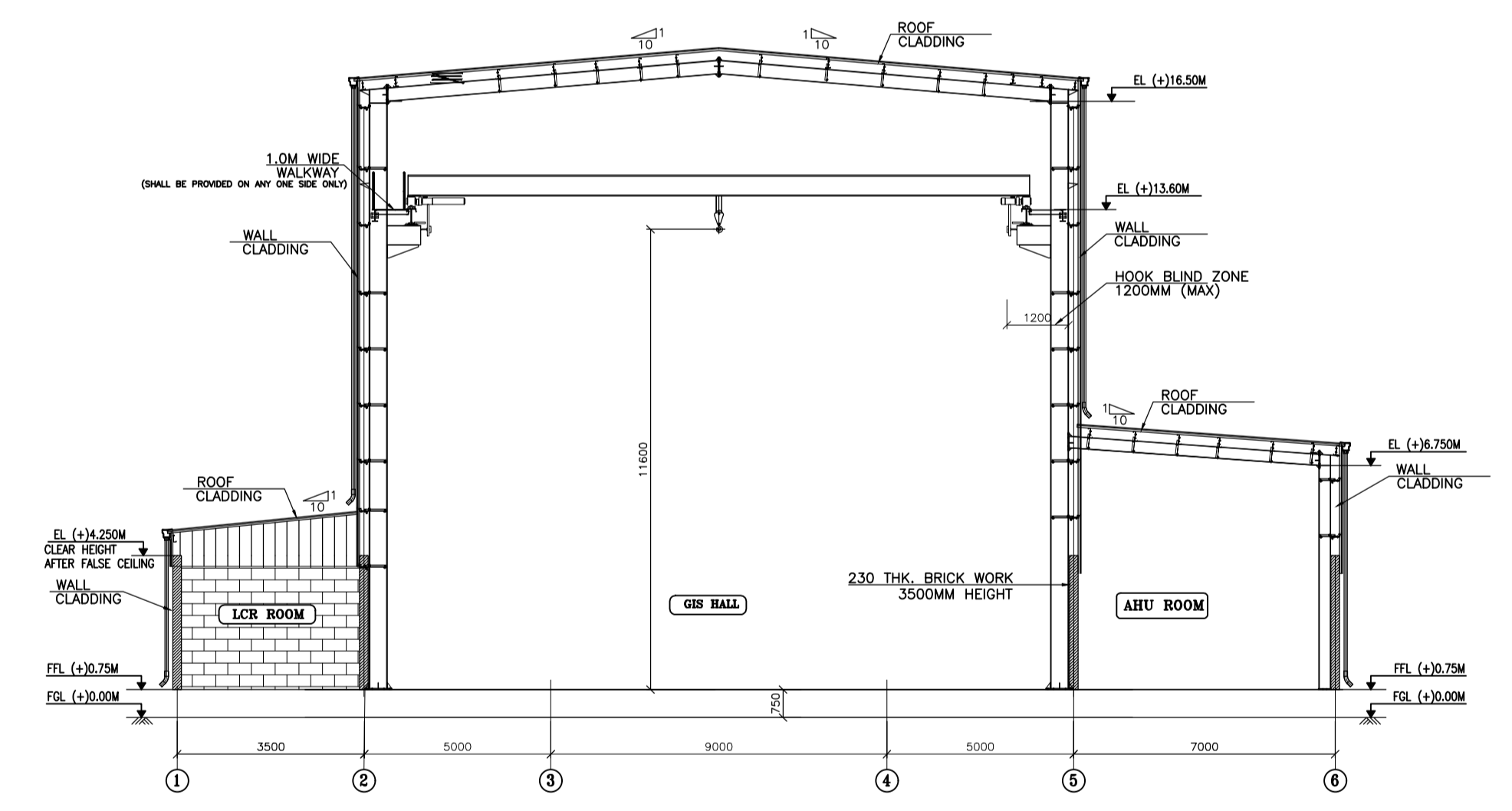
SECTION 1-1
