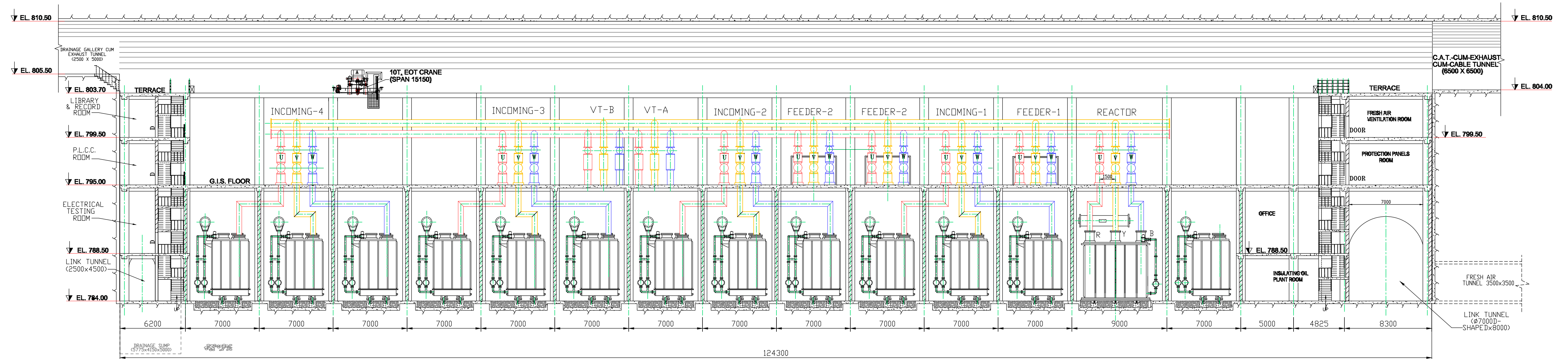
TRANSFORMER HALL LONGITUDINAL SECTION M-M
