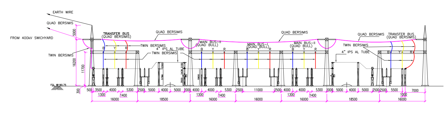
SECTION-J (220KV-TBC)
