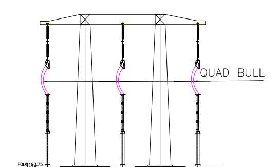
SECTION-L (765KV BUS CVT SECTION)
