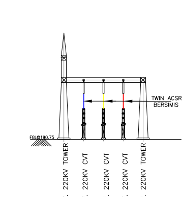
SECTION-N (220KV BUS CVT SECTION)
