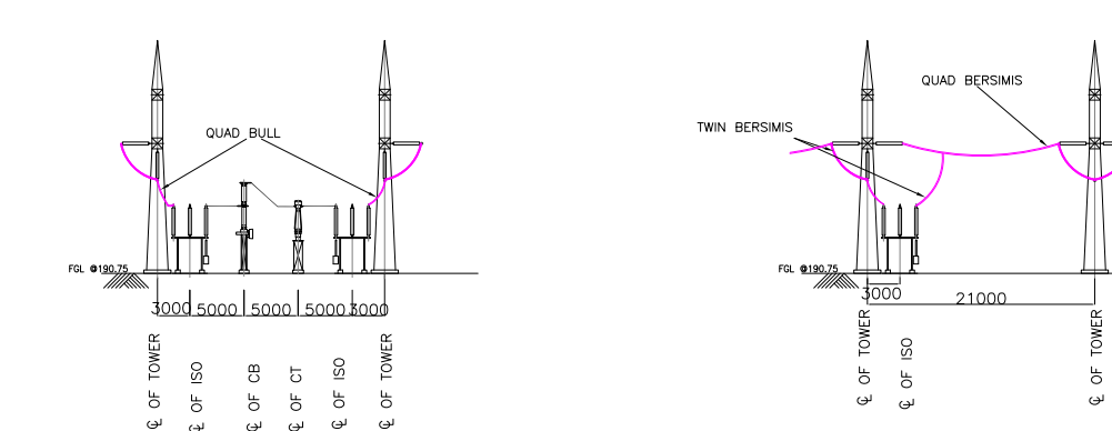
SECTION-O (220KV BUS SECTIONALIZER)
