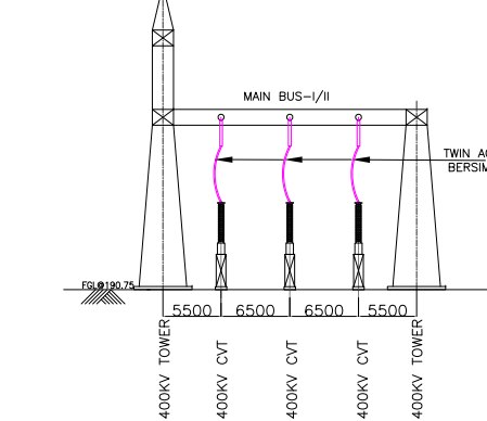
SECTION-M (400KV BUS CVT SECTION)
