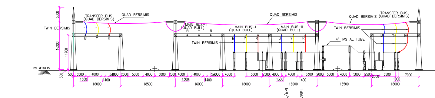
SECTION-I (220KV-BUS COUPLER-TIE-LINE)
