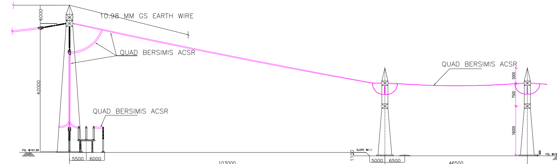
SECTION-V (220KV ICT-TIE-TBC-2)
