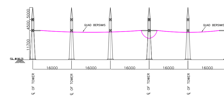
SECTION-T (220KV TRANSFER BUS)
