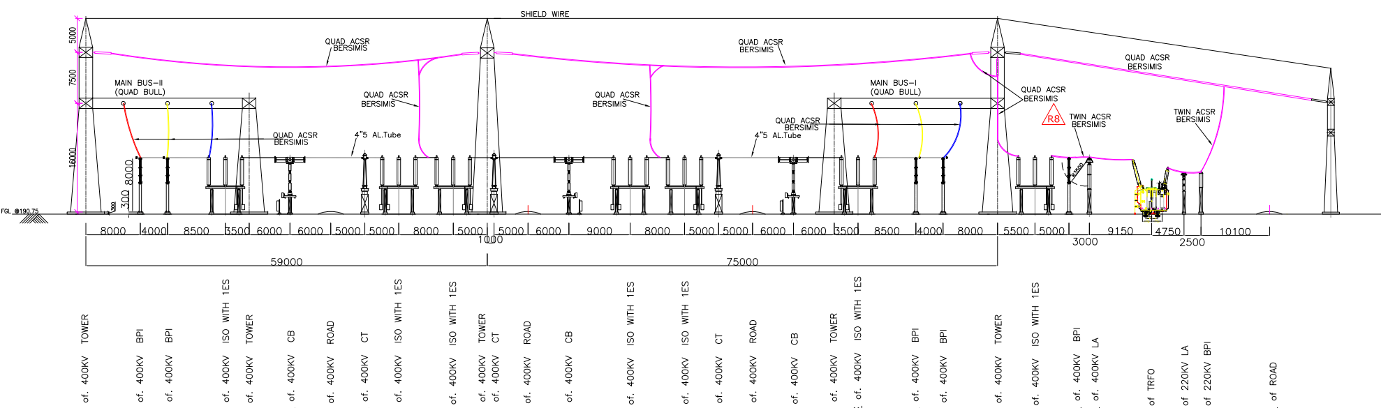
SECTION-F (400KV BAY-TIE-ICT)
