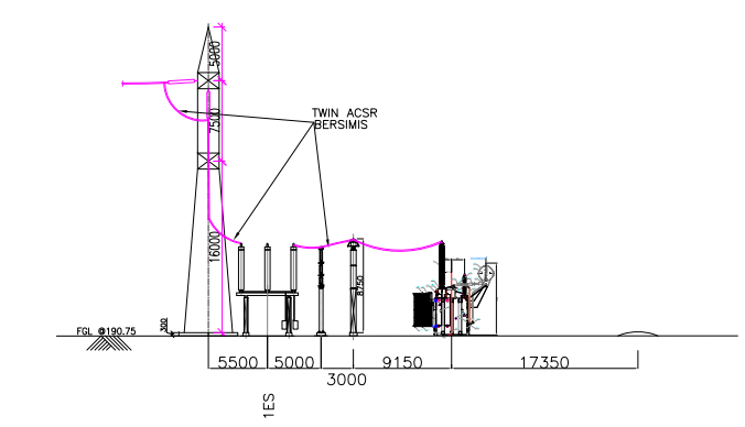
SECTION-K (765KV-400KV INTERCONNECTION)
