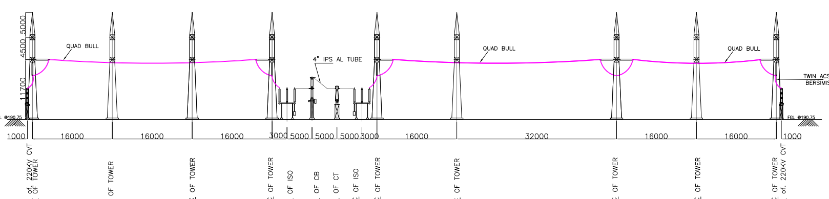
SECTION-S (220KV MAIN BUS-I/II)
