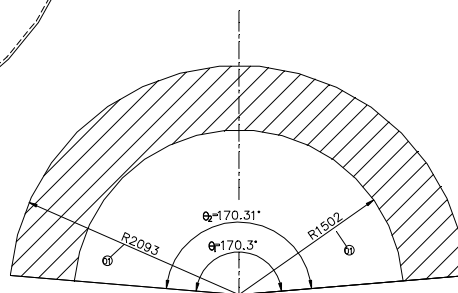
DEVELOPMENT OF CONE SCALE 1:50
