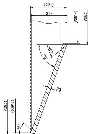
SECTION AA (A3) SCALE 1:5
