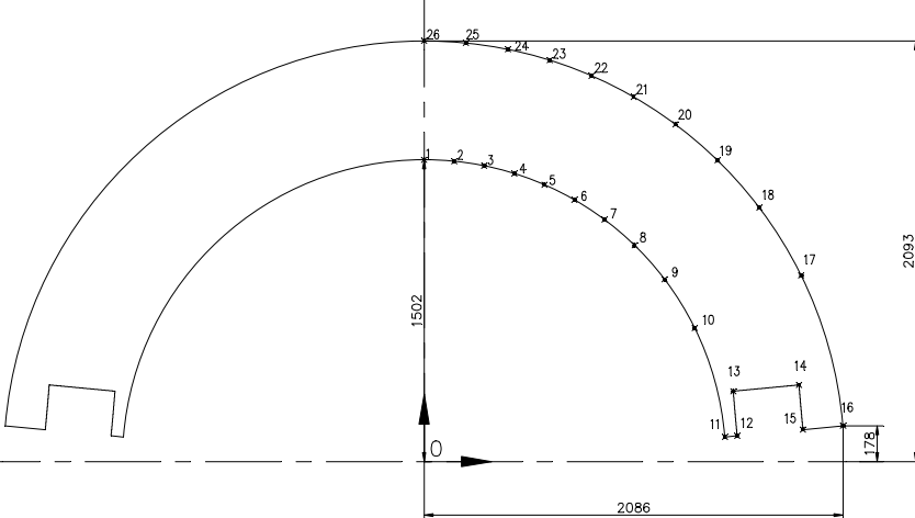
DEVELOPMENT OF CONE SCALE 1:15
