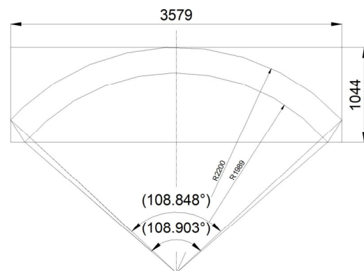
DEVELOPMENT (SCALE NTS)
