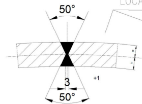
EDGE PREPARATION FOR WELD JOINTS (SCALE: NTS)
