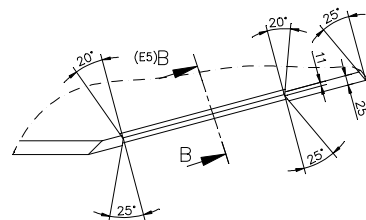
VIEW V (A4) SCALE 1:5
