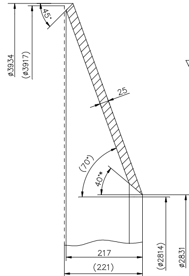
SECTION BB (A1) SCALE 1:5
