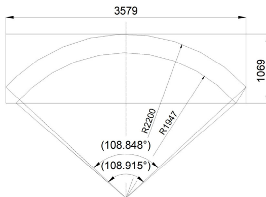
DEVELOPMENT (SCALE NTS)
