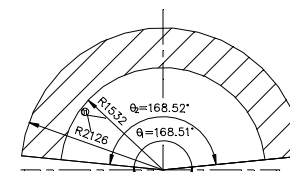
DEVELOPMENT OF CONE SCALE 1:150
