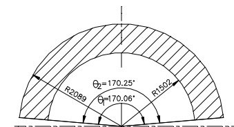
DEVELOPMENT OF CONE SCALE 1:50
