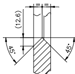
SECTION BB (D2) SCALE 1:2
