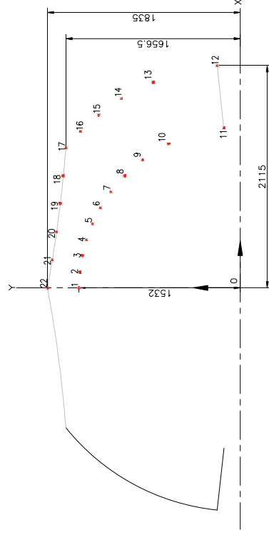
DEVELOPMENT OF CONE
