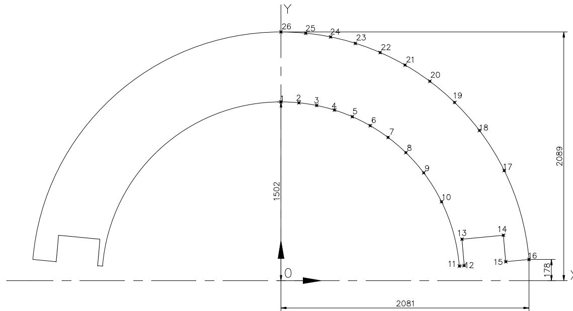
DEVELOPMENT OF CONE SCALE 1:50
