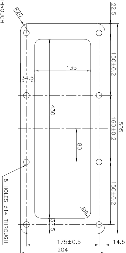
COACH SIDE FITMENT BASE PLATE ITEM-002
