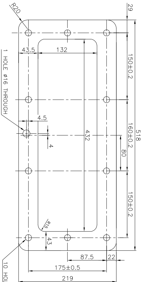
TRACTION MOTOR SIDE FITMENT BASE PLATE ITEM--001
