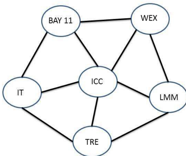
CORE SWITCH TO DISTRIBUTION CONNECTIVITY FOR BHEL JHANSI
