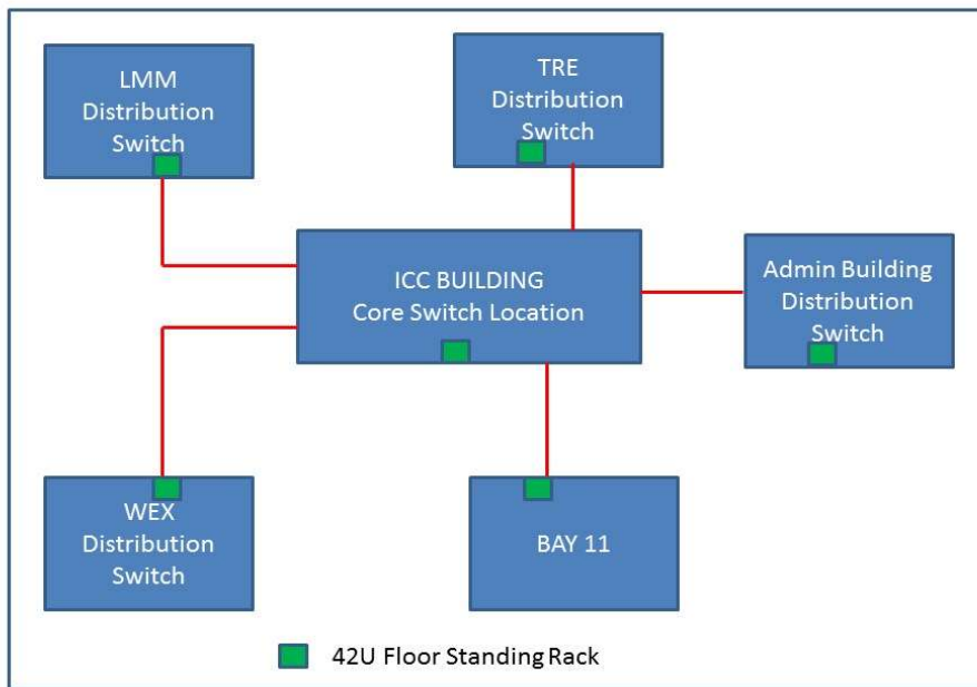
CORE SWITCH TO DISTRIBUTION CONNECTIVITY FOR BHEL JHANSI
