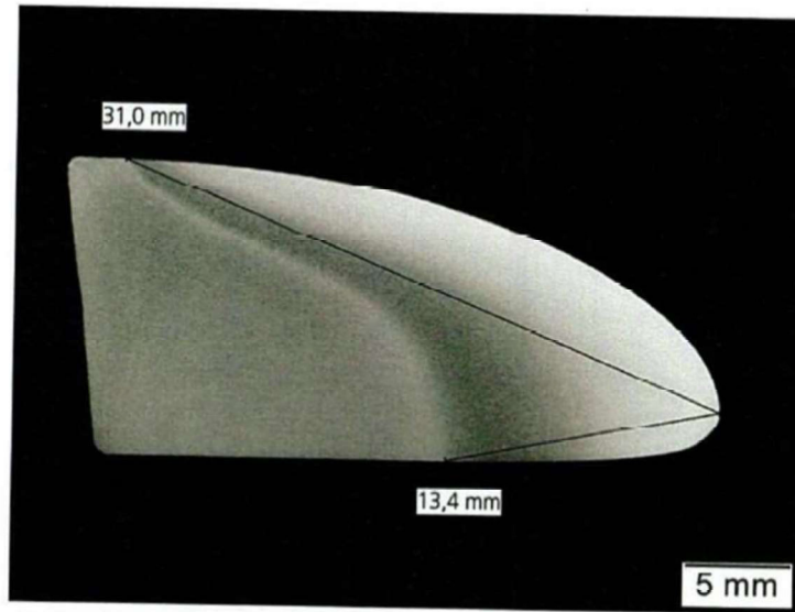
fig. 7: Cross section of a leading edge, hardened by laser assisted solution annealing followed by age hardening sample: CB-27-2.07; X=300
