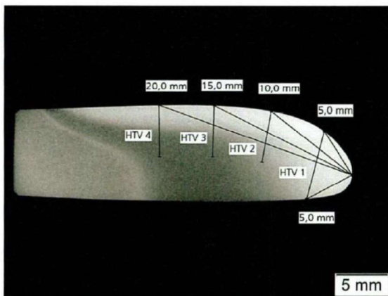
fig. 15: Position of the hardness lines sample: CB-27-2.02; X=50
