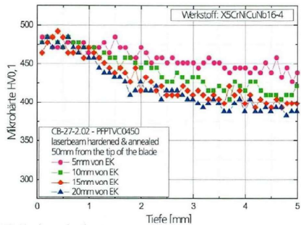
fig. 12: Hardness-depth-curve sample: CB-27-2.02; X=50
