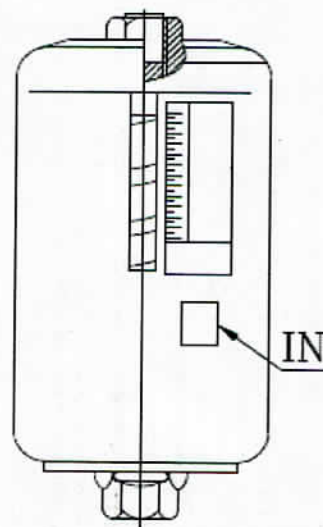
VARIABLE LOAD SPRING HANGER (TYPICAL SKETCH)
