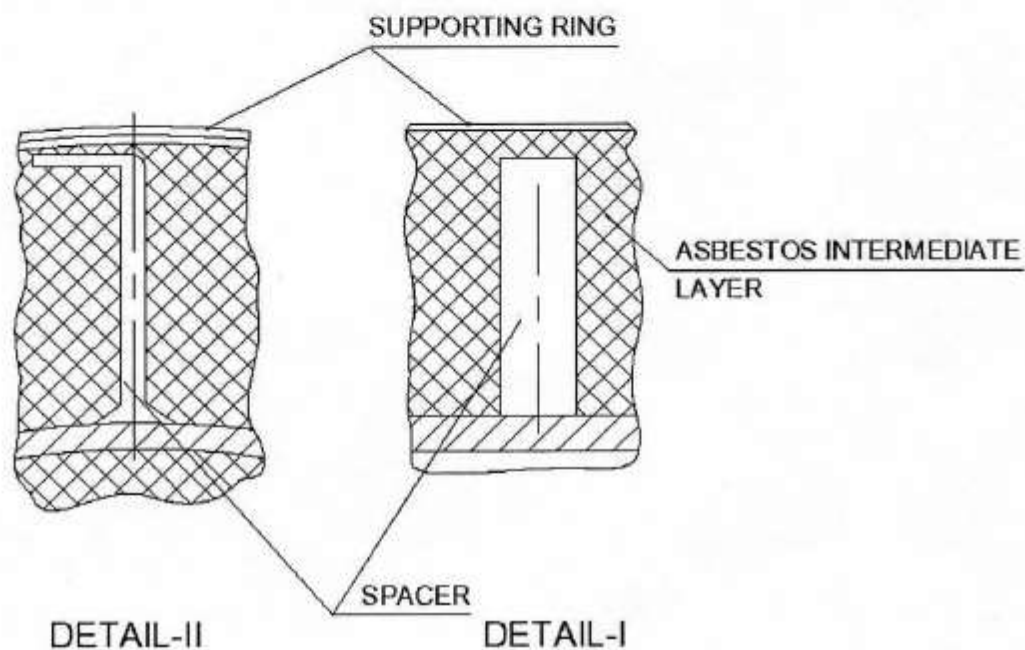
FIG.-5 STANDARD PIPE INSULATION
