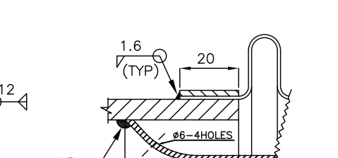
DETAIL-C
