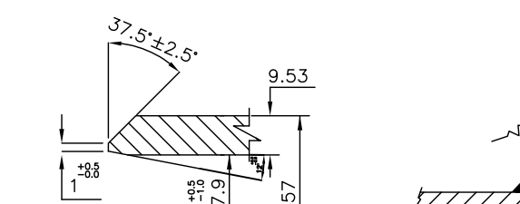
DETAIL-A
