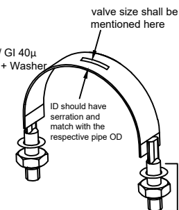
TYPICAL CLAMP
