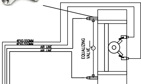
TYPICAL ACTUATOR TERMINALS
