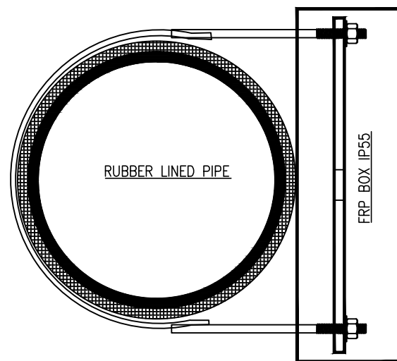
TYPICAL FRP JUNCTION BOX SIDE VIEW
