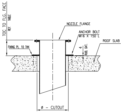
TYP. NOZZLE FIXING DETAIL
