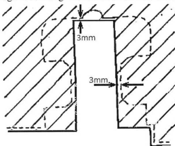
T- GROOVE ROUGH MACHINING
