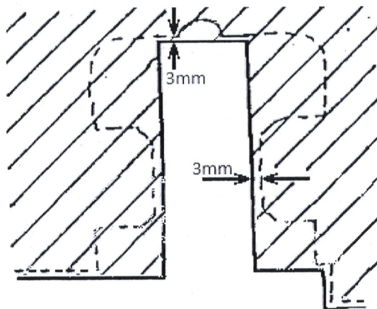
T- GROOVE ROUGH MACHINING
