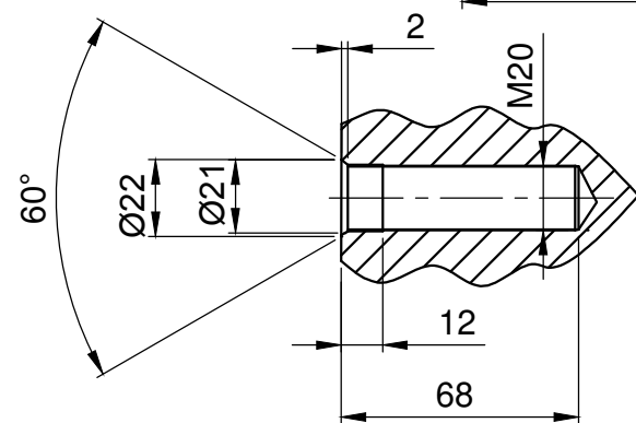
DETAIL - X
