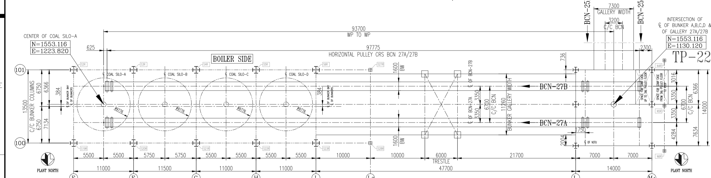
PLAN OF BCN 27A/27B
