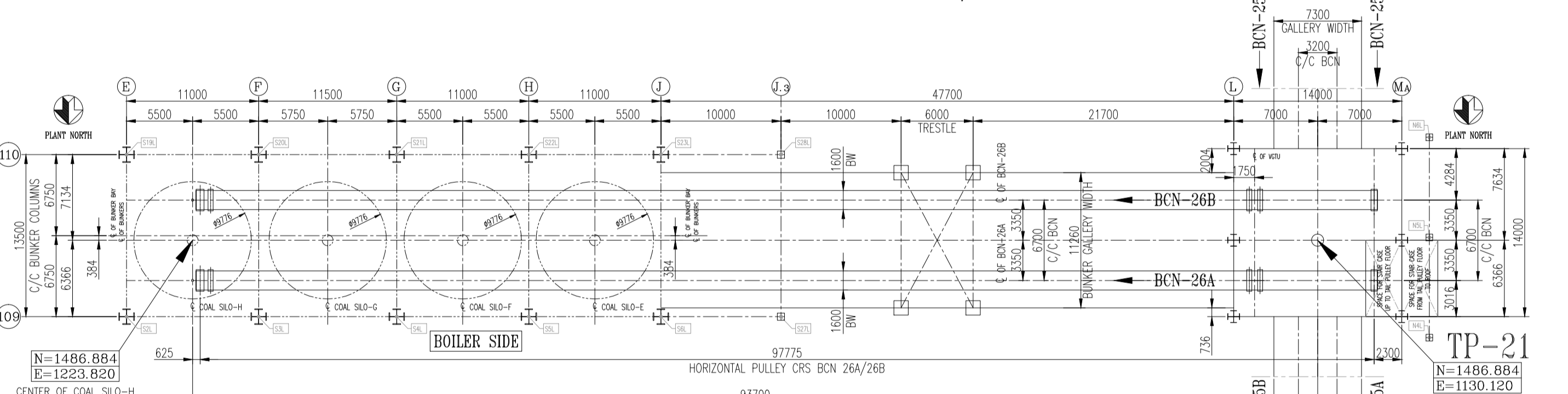
PLAN OF BCN 26A/26B
