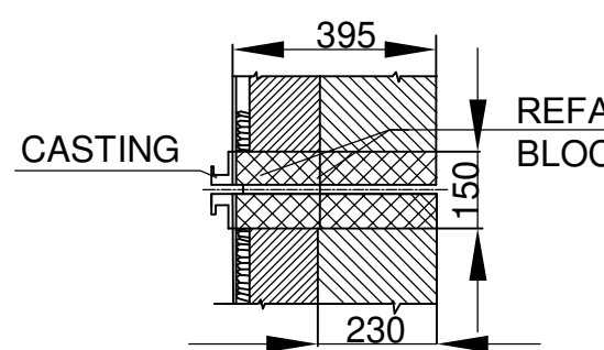
SECTION-QQ THERMOCOUPLE AND PRESSURE TAPPING AT SIDE WALL
