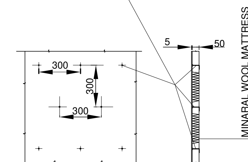
MATTRESS HOLDING DETAIL
