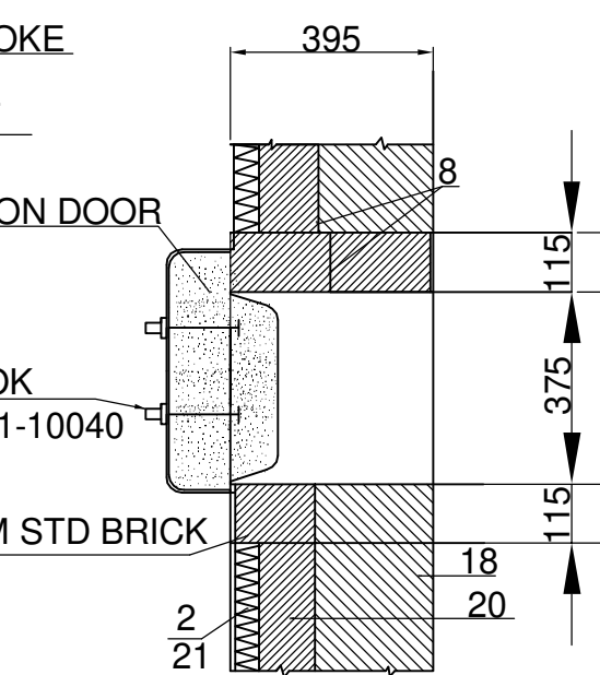
SECTION-PP
