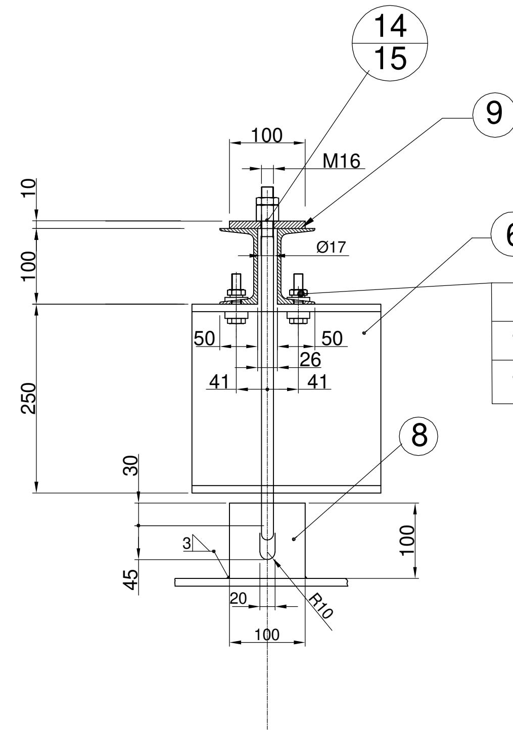
DETAIL 'Y'
