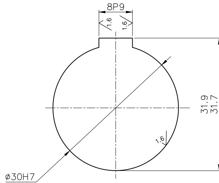
KEYWAY-DETAILS
