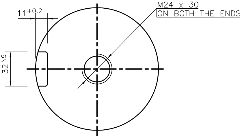
VIEW-X SCALE-1:2
