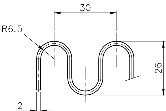
DETAIL-X
