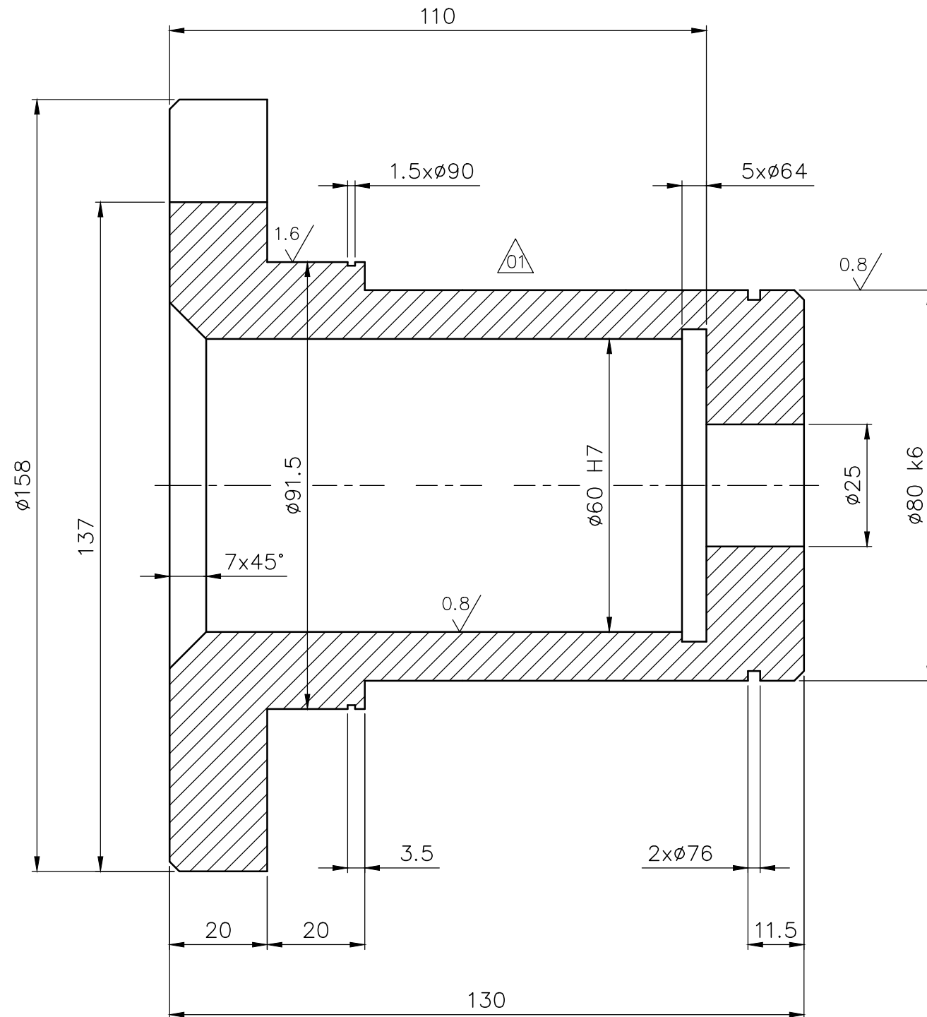
SECTION - 'AA'
