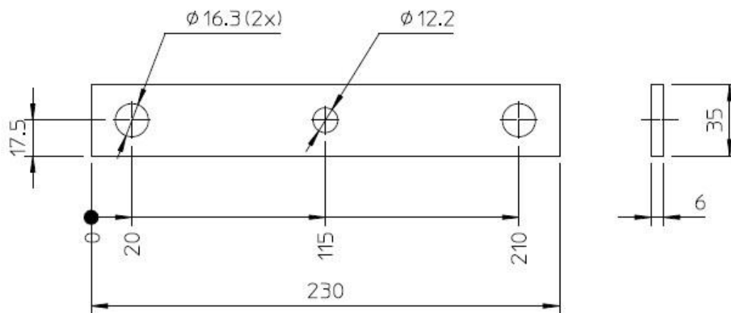
Drawing 1: Strip
