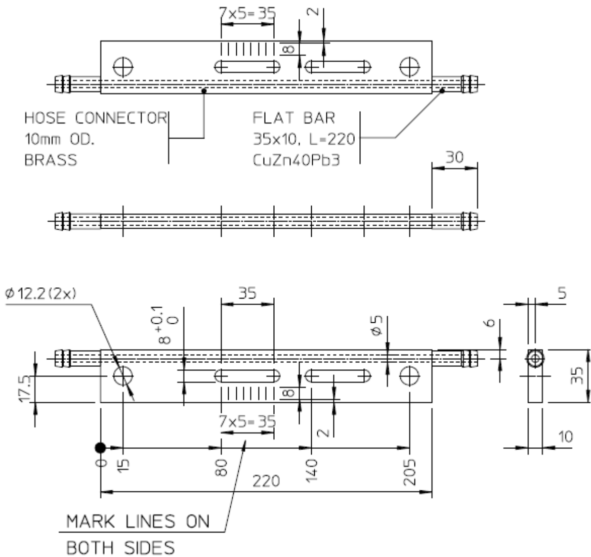
Drawing 2:Strip
