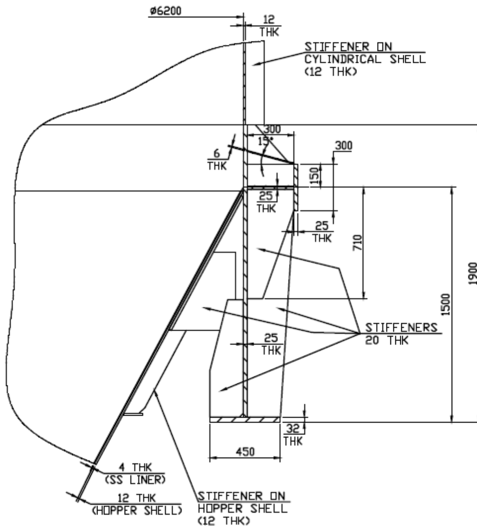
RING GIRDER (CONSTRUCTION DETAIL)
