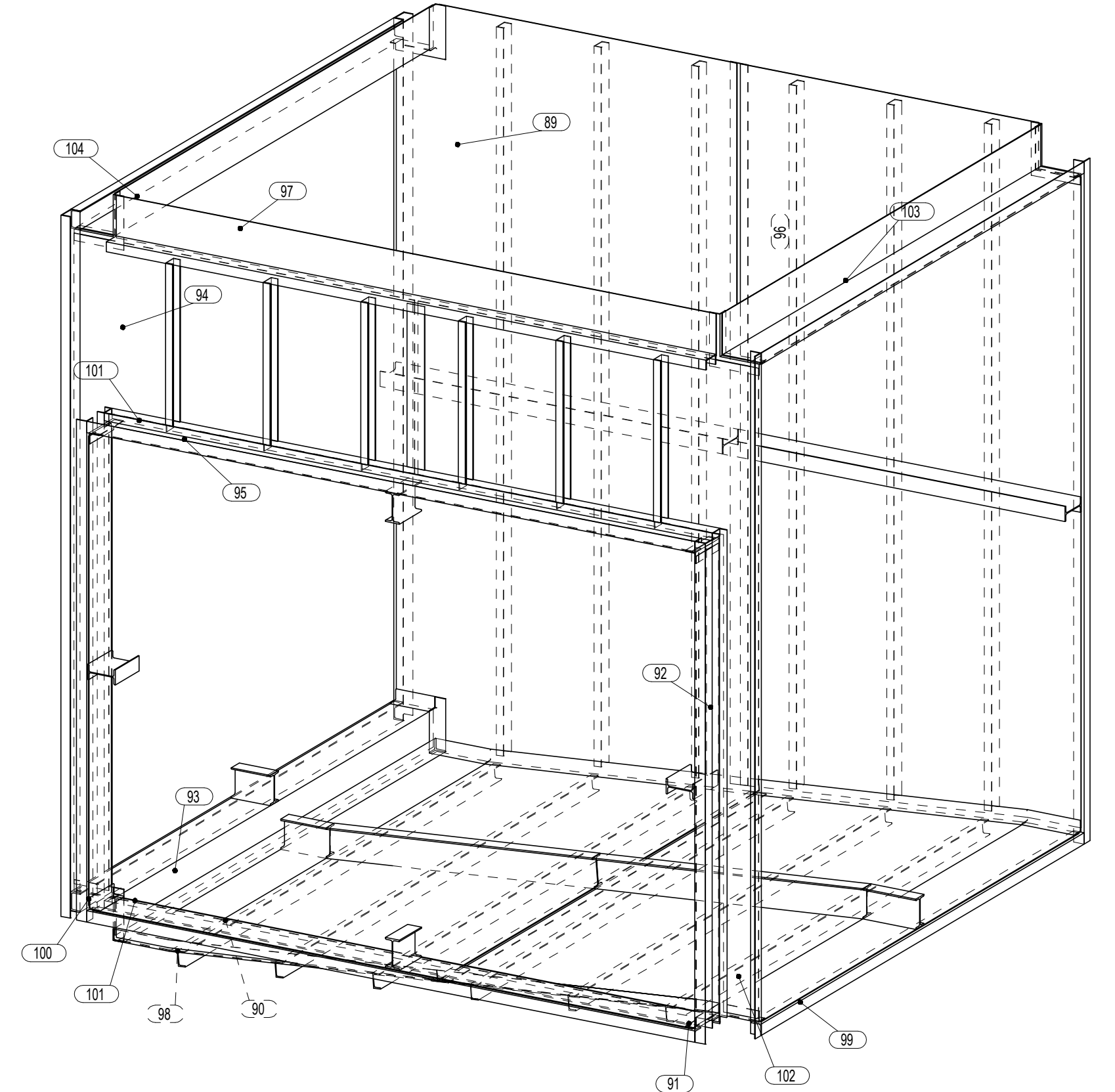
ISOMETRIC
