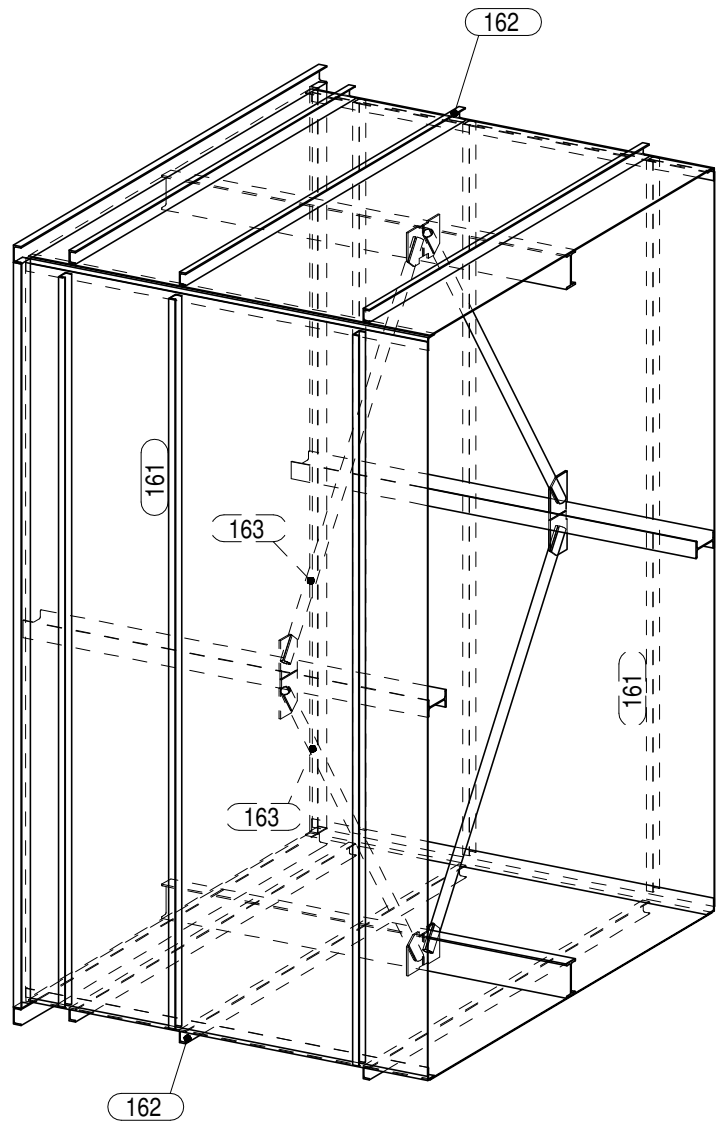
ISOMETRIC
