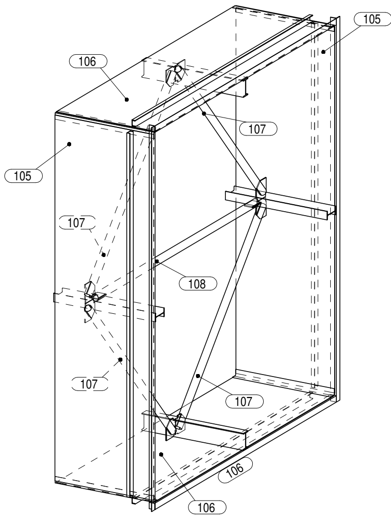
ISOMETRIC
