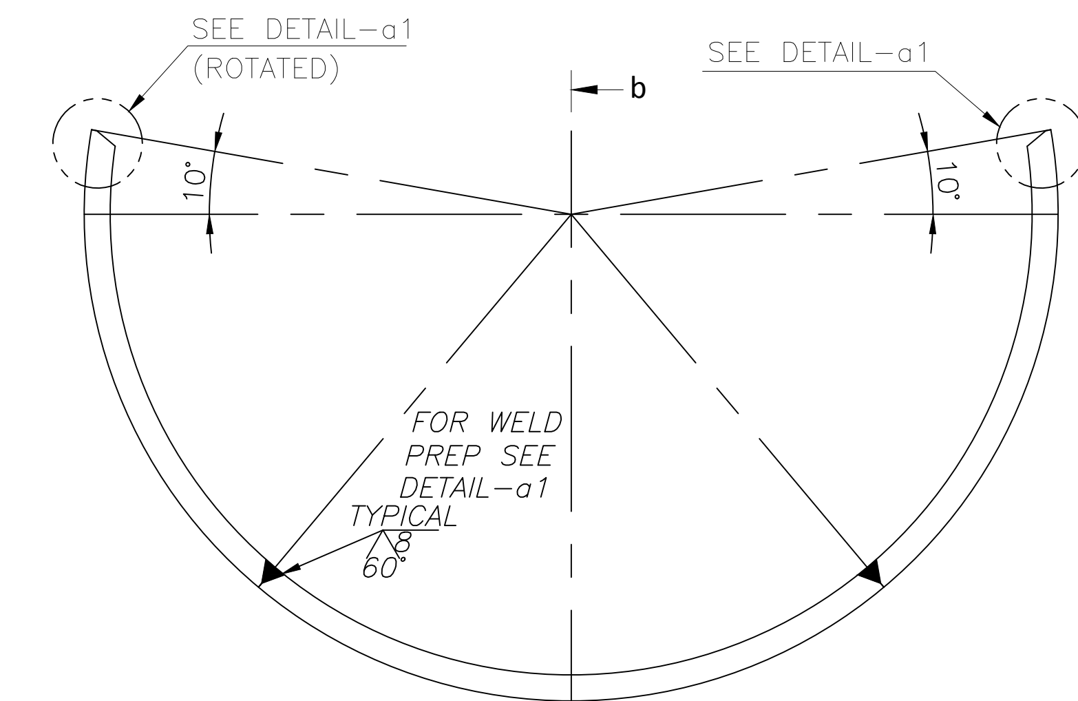
DETAIL OF ITEM-03 NTS
