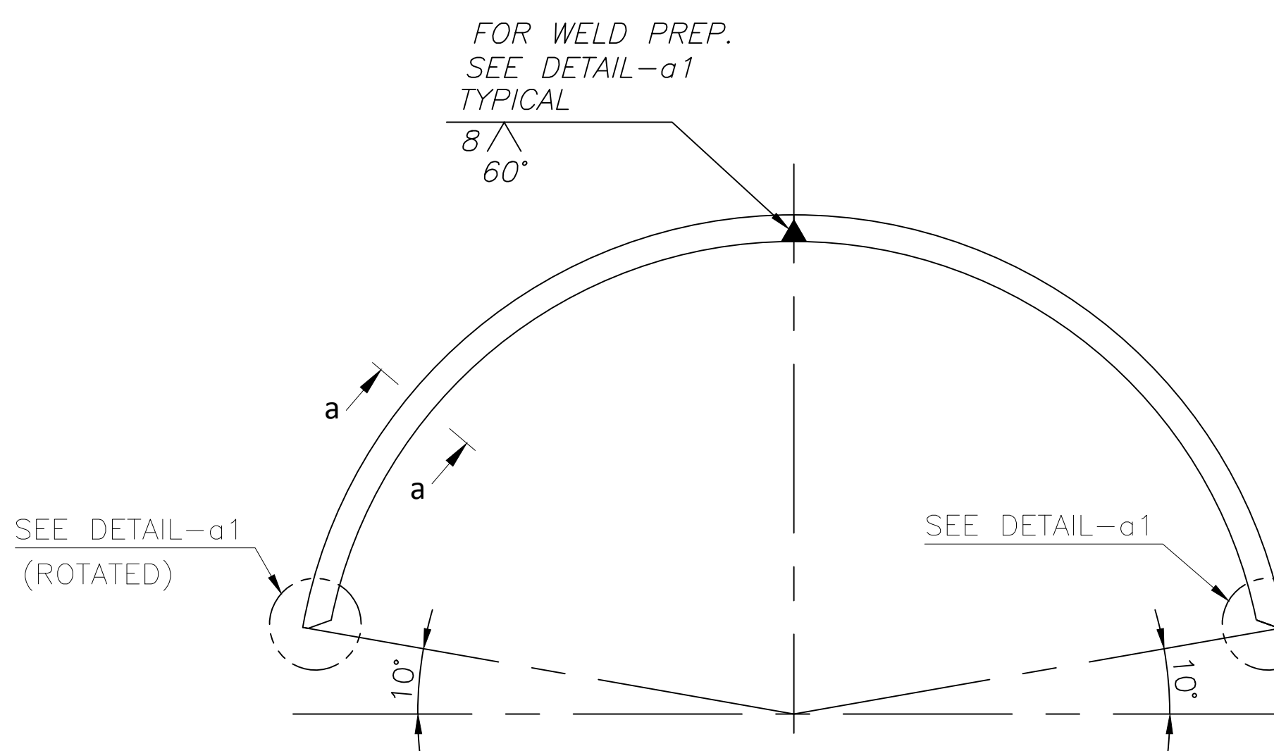
DETAIL OF ITEM-02 & 08 NTS
