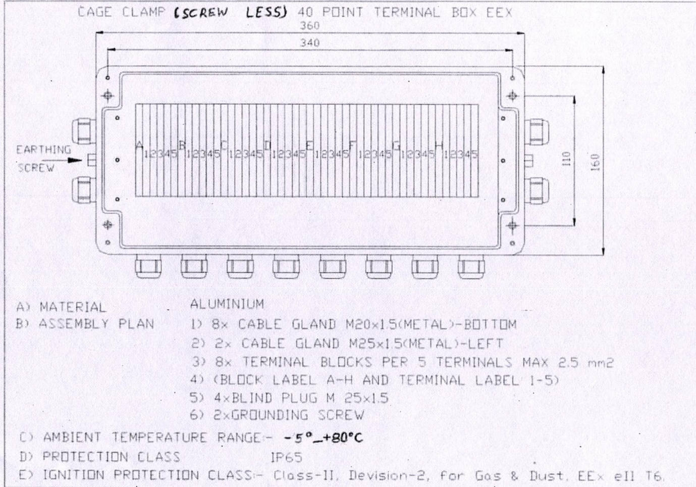
Fig -3 : Field Junction box.
