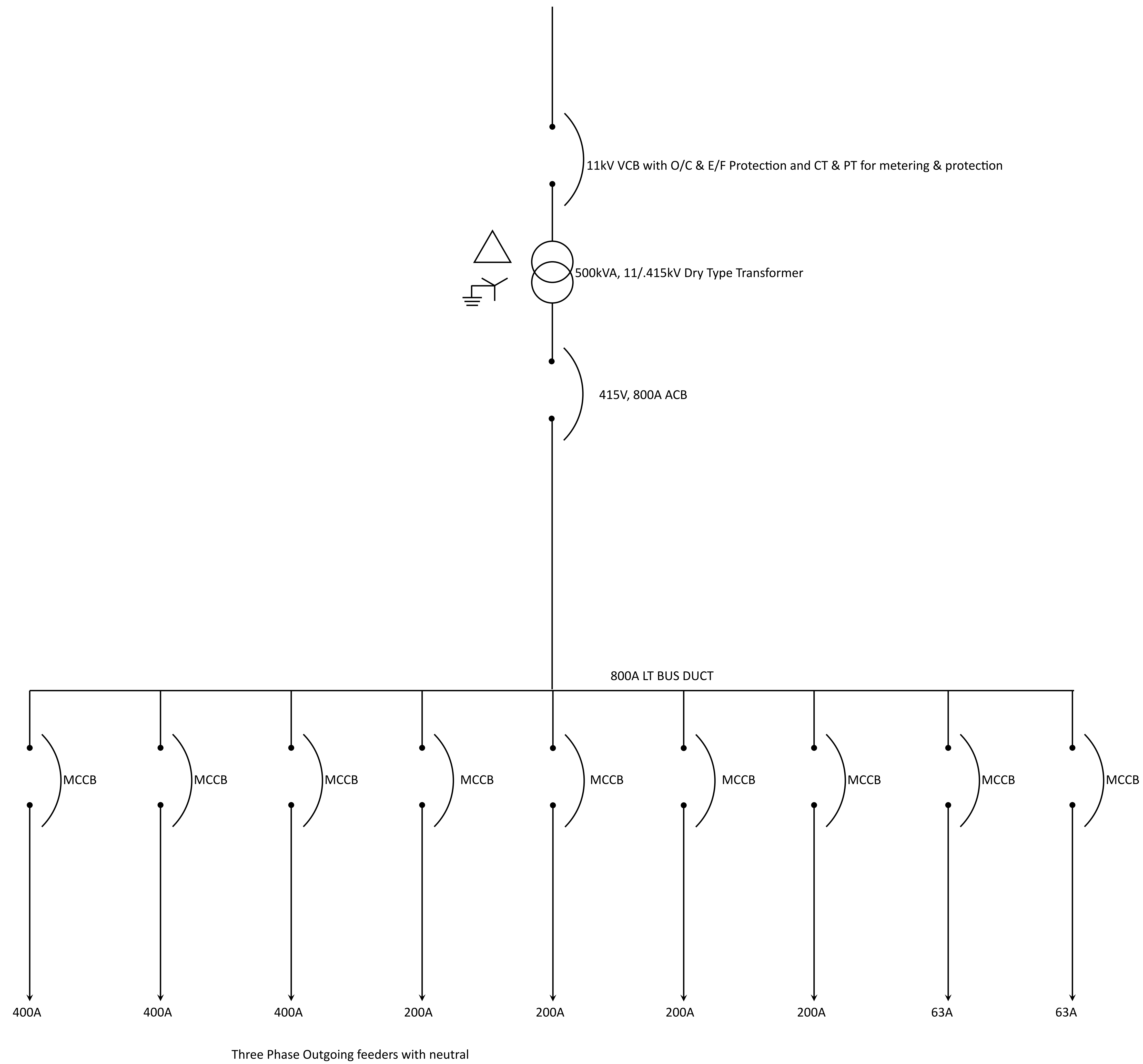
Single Line Diagram of 500kVA Package Substation
