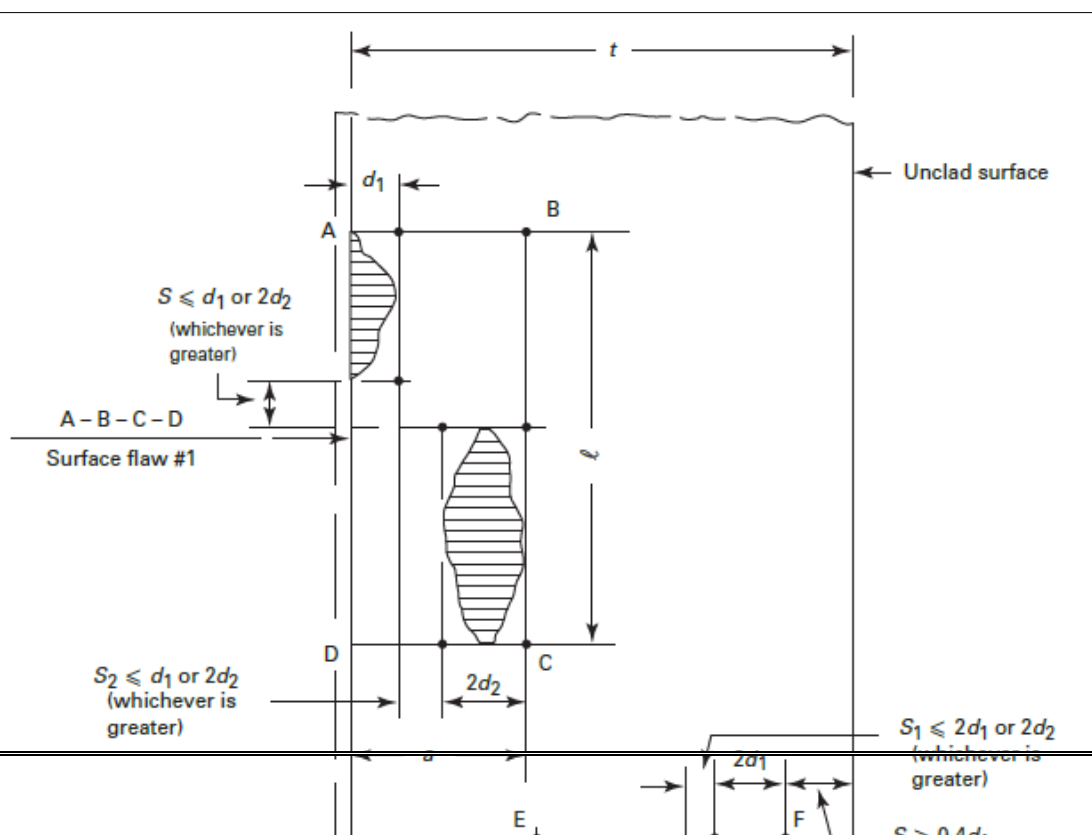
Nonaligned Coplanar Flaws in Plane Normal to Pressure Retaining Surface (Illustrative Flaw Configurations)
