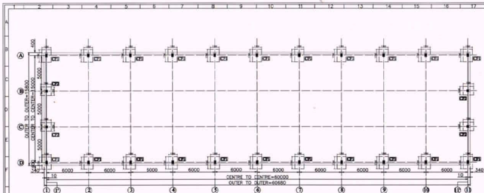
FOUNDATION PLAN
